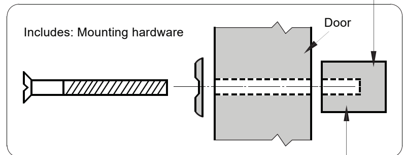
SCHPH-4000-2 OFFSET DOOR PULL SET
