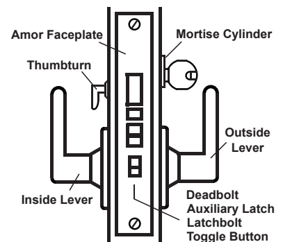
ANSI Function Diagram
